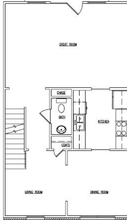
MAIN LEVEL
